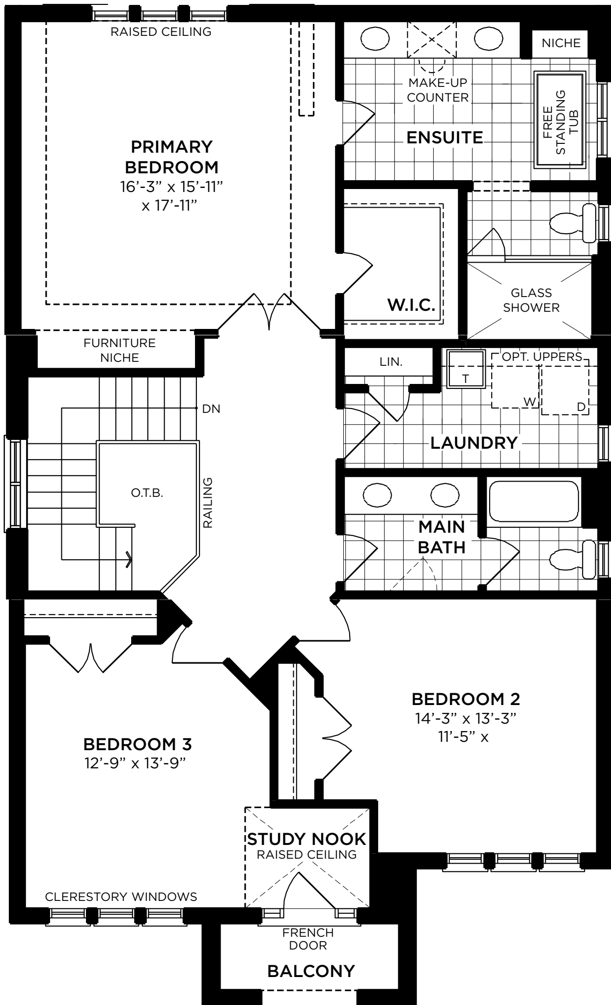
PART. OPT. SECOND FLOOR PLAN W/ 3 BEDROOM Elev. B
